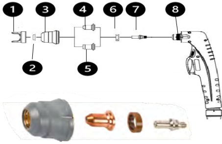
Forney® 20P, Flex™ 30 and 40P Consumables
